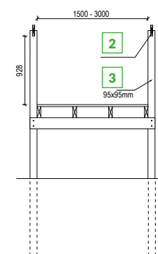
CORTE TRANSVERSAL COUPE TRANSVERSALE CROSS-SECTION
